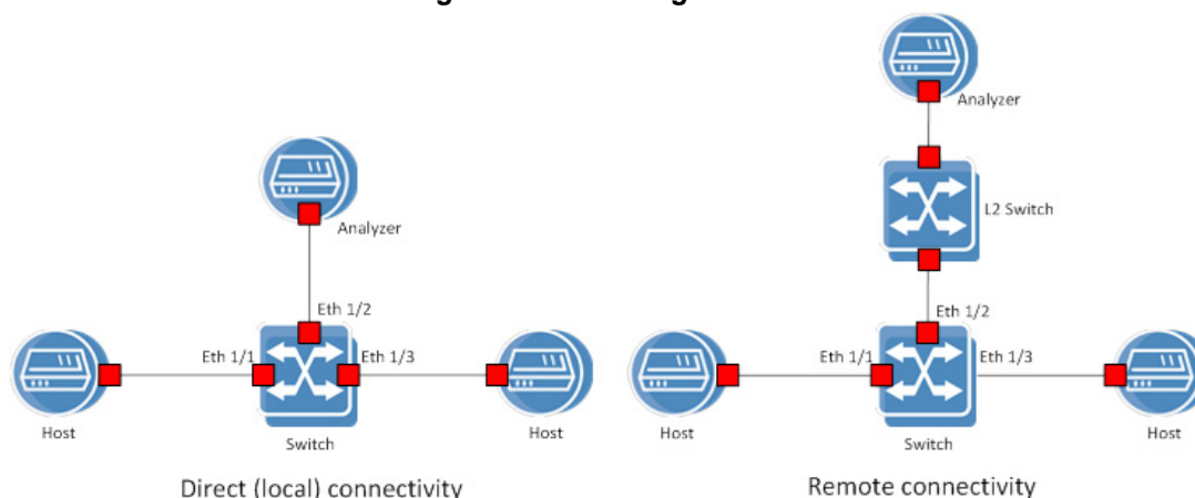
Figure 23: Mirroring Session
