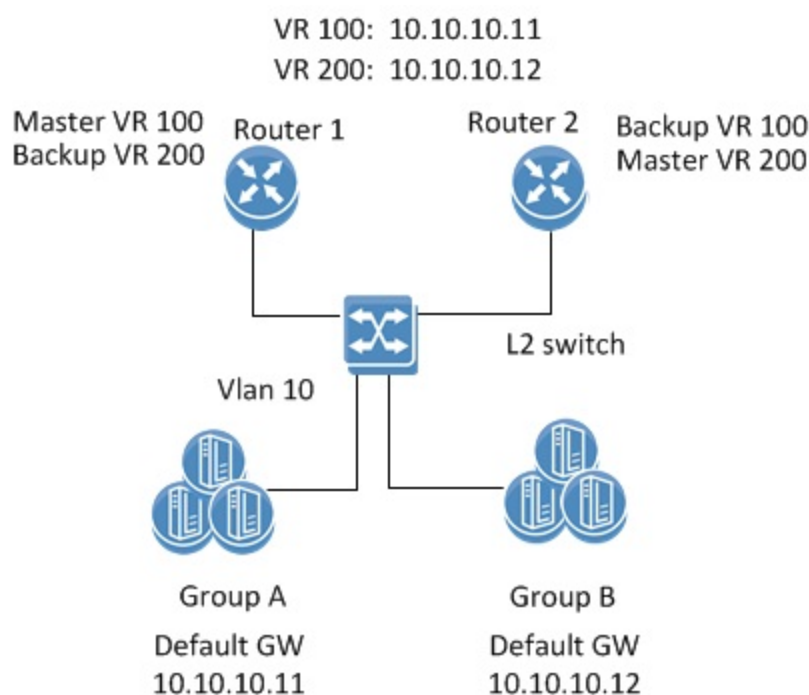
Figure 33: Common VRRP Configuration with Load Balancing
