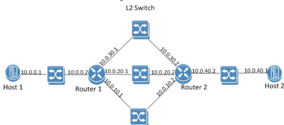
Figure 28: ECMP
