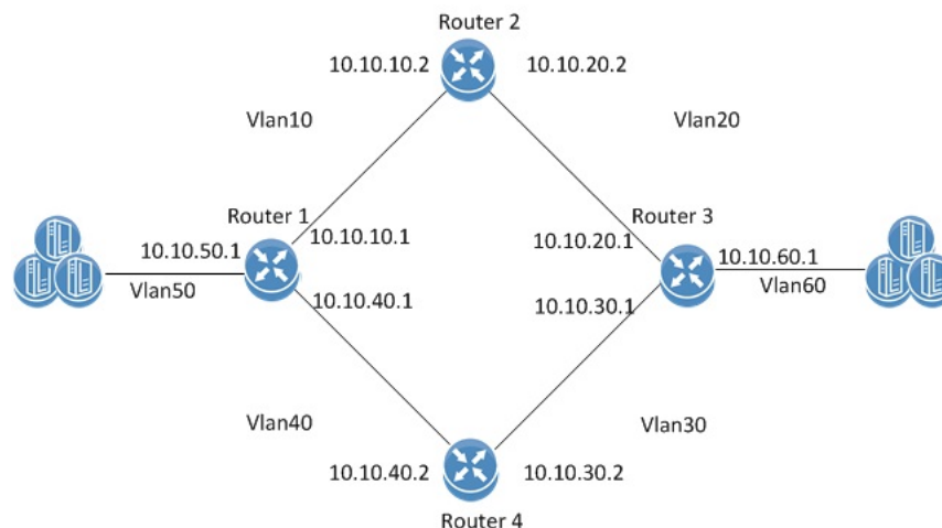
Figure 31: OSPF Basic Topology
