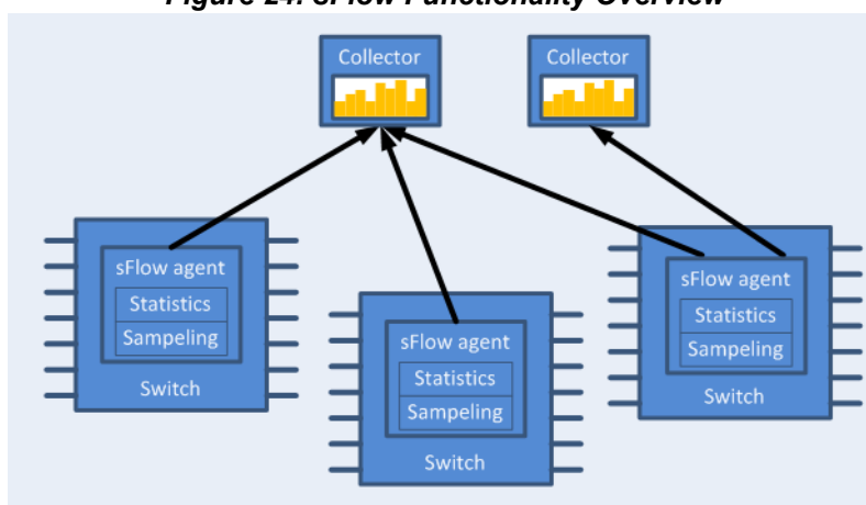
Figure 24: sFlow Functionality Overview
