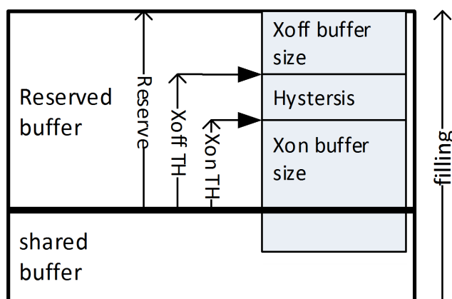
Figure 27: Xon/Xoff Configuration
