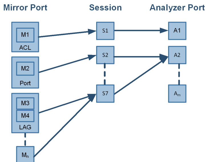
Figure 21: Mirror to Analyzer Mapping
