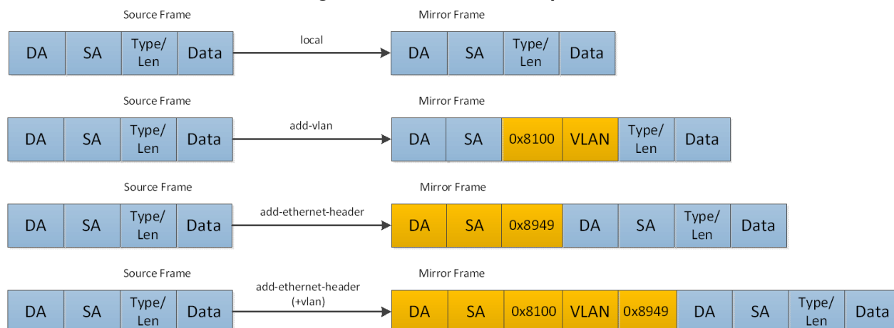
Figure 22: Header Format Options
