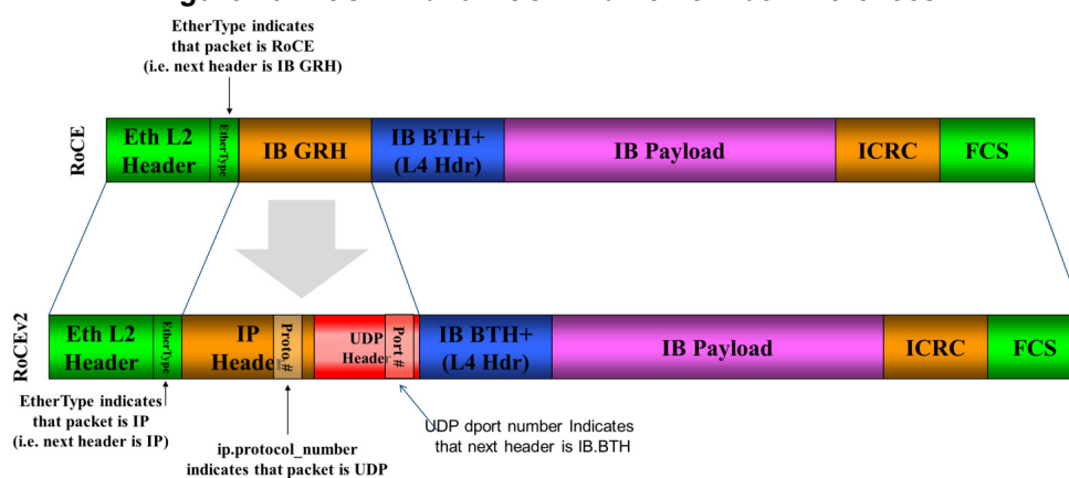
Figure 25: RoCEv2 and RoCE Frame Format Differences
