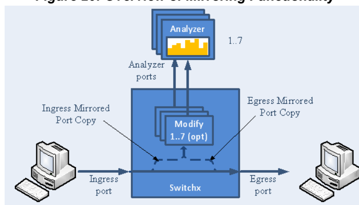
Figure 20: Overview of Mirroring Functionality
