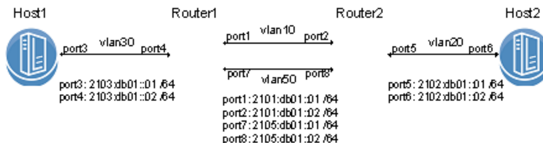
Figure 30: IPv6 Network
