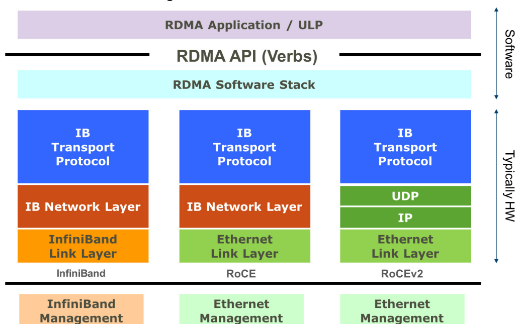
Figure 26: RoCEv2 Protocol Stack
