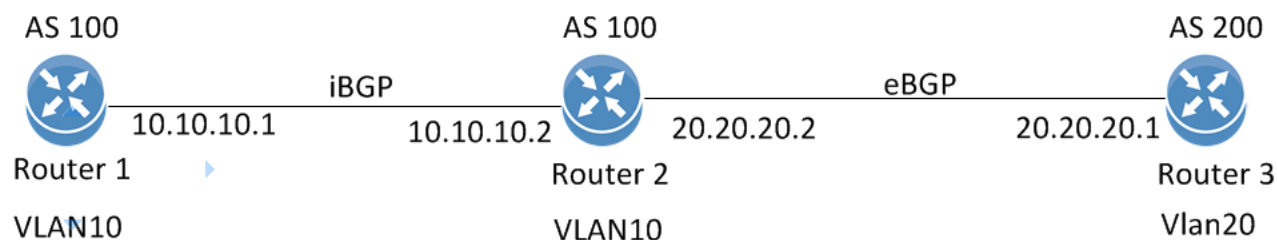
Figure 32: Basic BGP Configuration
