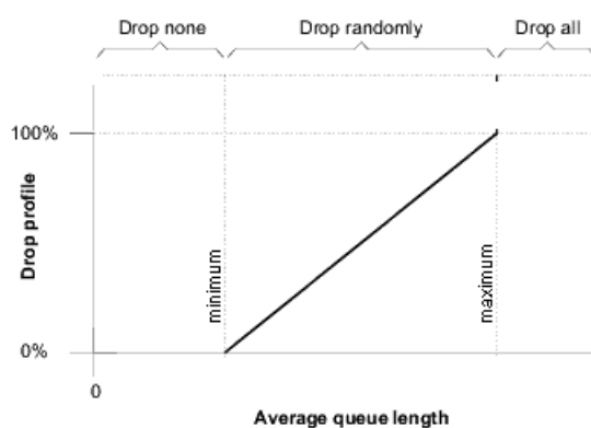
Figure 19: RED/ECN Drop Profiles
